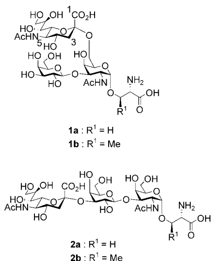
Scheme 1. Structures of 2,6- and 2,3-sialyl Tantigens 1 and 2 .
