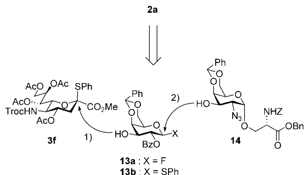
Scheme 5. Strategy for the one-pot two-step synthesis of 2a .
