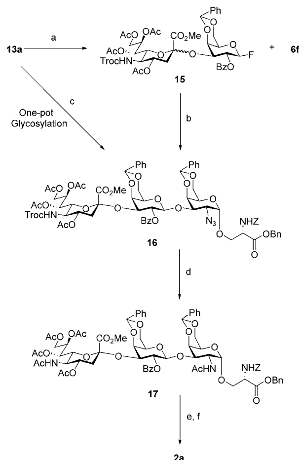
Scheme 6. Synthesis of 2,3-sialyl T antigen 2a by a stepwise process and by a linear-type one-pot glycosylation. Reagents and conditions: a) 3f (1.50 equiv), NIS (2.00 equiv), TfOH (0.30 equiv), CH 3 CN/CH 2 Cl 2 (2:3; 5 mL mmol -1 ), 3 Å MS (0.50 g mmol -1 ), -78 °C, 86%, \alpha : \beta =93:7; b) 14 (1.30 equiv), ZrCp 2 Cl 2 (1.50 equiv), AgOTf (3.00 equiv), CH 3 CN/CH 2 Cl 2 (2:3; 5 mL mmol -1 ), 3 Å MS (0.50 g mmol -1 ), -5 °C, 96%; c) 3f (1.50 equiv), 13a (1.00 equiv), NIS (2.00 equiv), TfOH (0.30 equiv), CH 3 CN/CH 2 Cl 2 (2:3; 5 mL mmol -1 ), 3 Å MS (0.50 g mmol -1 ), -78 °C; then 14 (1.50 equiv), ZrCp 2 Cl 2 (2.00 equiv), AgOTf (4.00 equiv), -5 °C, 88%, \alpha : \beta =93:7; d) Zn dust, THF, AcOH, Ac 2 O, 0 °C, 1 h, 93%; e) Pd(OH) 2 , THF, MeOH, AcOH, H 2 O, 2 h; f) 0.1 N NaOH, MeOH; then H 2 O, 90% over two steps.
