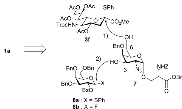
Scheme 3. Strategy for the one-pot two-step synthesis of 1a . Bz = benzoyl.
