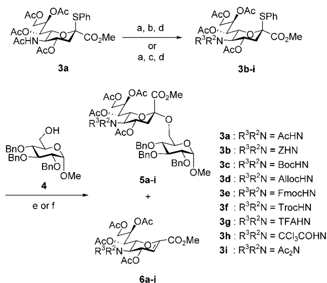
Scheme 2. Synthesis and glycosidation of \beta -thiophenyl sialosides 3a–i . Reagents and conditions: a) MsOH, MeOH, 60°C, 12 h; b) Z-OSu, Alloc-OSu, Fmoc-OSu, Troc-OSu, or (Boc) 2 O, NEt 3 , CH 3 CN/H 2 O, RT, 5.5 h; c) CF 3 CO 2 Me or CCl 3 CO 2 Me, NEt 3 , MeOH, RT, 1 h; d) Ac 2 O, Py, DMAP, 63% for 3b , 76% for 3c , 68% for 3d , 27% for 3e , 89% for 3f , 77% for 3g , and 70% for 3h in three steps from 3a ; e) 3a–i (1.00 equiv), 4 (1.50 equiv), NIS (1.20 equiv), TfOH (0.20 equiv), CH 3 CN, 3 Å MS (10 gmmol −1 ), −35°C, 1 h; f) 3a–i (1.00 equiv), 4 (1.50 equiv), DMTST (1.50 equiv), CH 3 CN, 3 Å MS (10 gmmol −1 ), −10°C, 8 h. Alloc = allyloxycarbonyl, Bn = benzyl, Boc = tert -butoxycarbonyl, DMAP = 4-dimethylaminopyridine, DMTST = (dimethylthio)methylsulfonium trifluoromethanesulfonate, Fmoc = 9-fluorenylmethoxycarbonyl, MsOH = methanesulfonic acid, NIS = N -iodosuccinimide, Py = pyridine, Su = succinimidyl, Tf = trifluoromethanesulfonyl, TFA = trifluoroacetyl, Troc = 2,2,2-trichloroethoxycarbonyl, Z = benzyloxycarbonyl.
