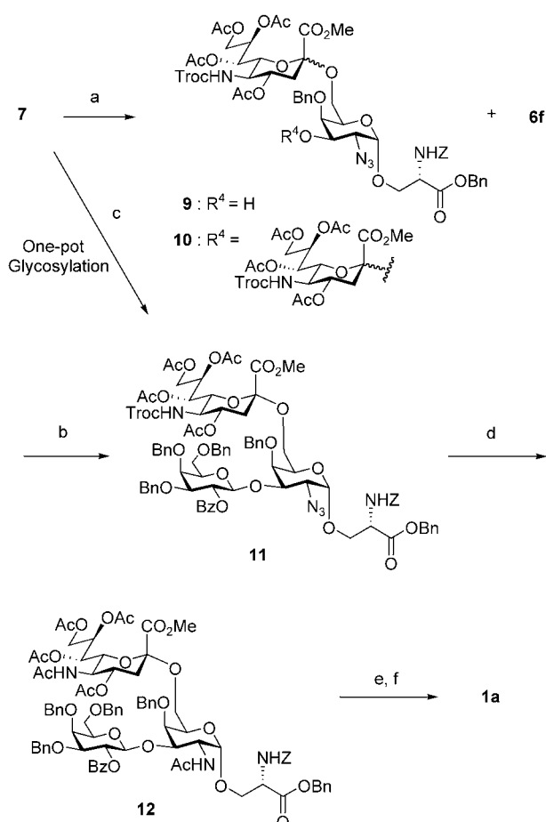
Scheme 4. Synthesis of 2,6-sialyl T antigen 1a by a stepwise process and by a branched-type one-pot glycosylation. Reagents and conditions: a) 3f (1.20 equiv), NIS (1.44 equiv), TfOH (0.10 equiv), CH 3 CN (5 mL mmol -1 ), 3 Å MS (0.50 g mmol -1 ), -35 °C, 93 %, α:β = 78:22; b) 8a (1.50 equiv), NIS (2.00 equiv), TfOH (0.20 equiv), CH 2 Cl 2 /CH 3 CN (9:1, 5 mL mmol -1 ), 3 Å MS (0.50 g mmol -1 ), -30 °C, 82 %, α:β = 6:94; c) 3f (1.20 equiv), 7 (1.00 equiv), NIS (1.44 equiv), TfOH (0.10 equiv), CH 3 CN (5 mL mmol -1 ), 3 Å MS (0.50 g mmol -1 ), -35 °C; then 8a (1.80 equiv), NIS (2.70 equiv), TfOH (0.20 equiv), CH 2 Cl 2 (45 mL mmol -1 ), -30 °C, 77 %, α:β = 78:22; d) Zn dust, THF, AcOH, Ac 2 O, 0 °C, 1 h, 92 %; e) Pd(OH) 2 , THF, MeOH, AcOH, H 2 O, 2 h; f) 0.1 M aq. NaOH, MeOH; then H 2 O, 85 % over two steps. THF = tetrahydrofuran.
